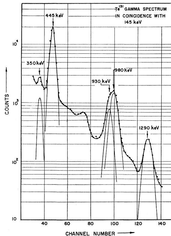
FIG. 2. Gamma spectrum in coincidence with the 145-keV transition.
