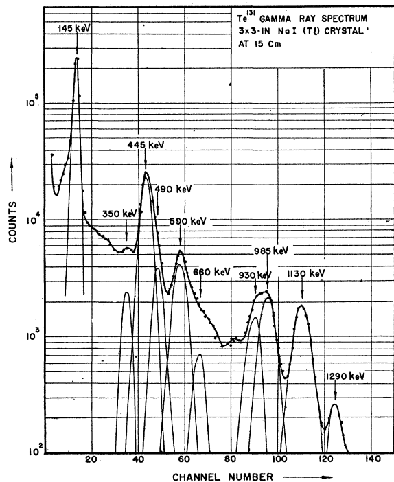
FIG. 1. Gamma spectrum of \text{Te}^{131} .
