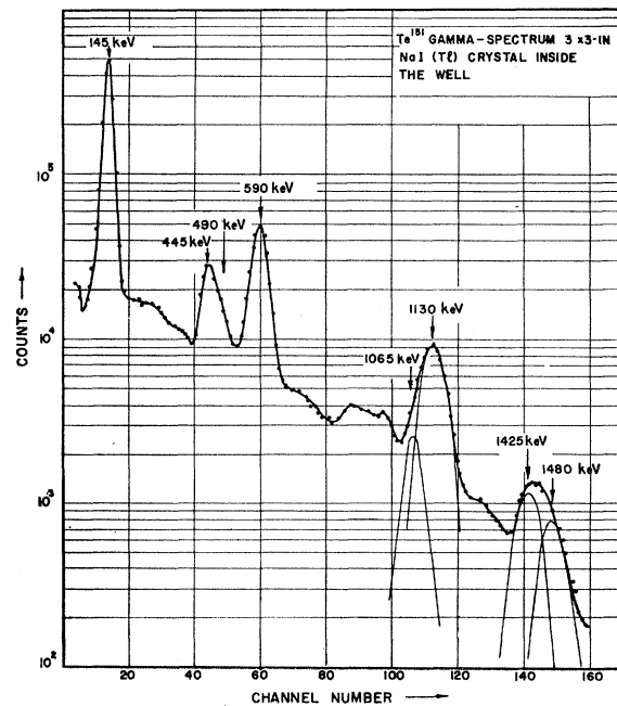
FIG. 4. Total absorption gamma spectrum of \text{Te}^{131} .
